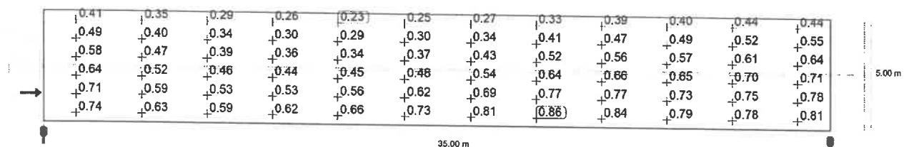
Observer 1: Maintenance value, luminance with dry roadway [ \text{cd}/\text{m}^2 ] (Value grid)
