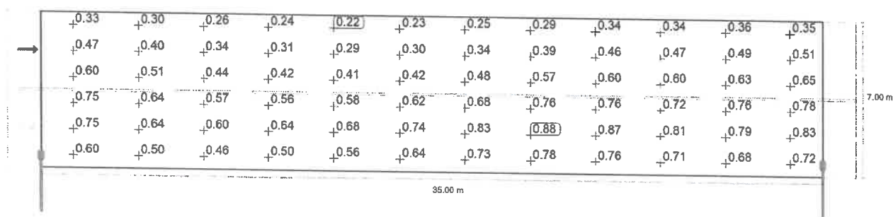
Observer 2: Maintenance value, luminance with dry roadway [ \text{cd/m}^2 ] (Value grid)
