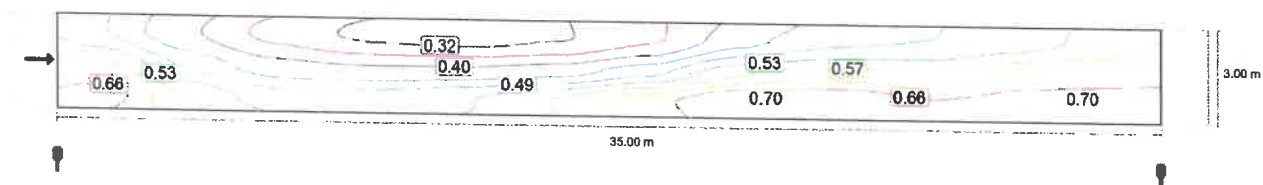
Observer 1: Luminance with new installation [cd/m²] (Iso-illuminance curves)
