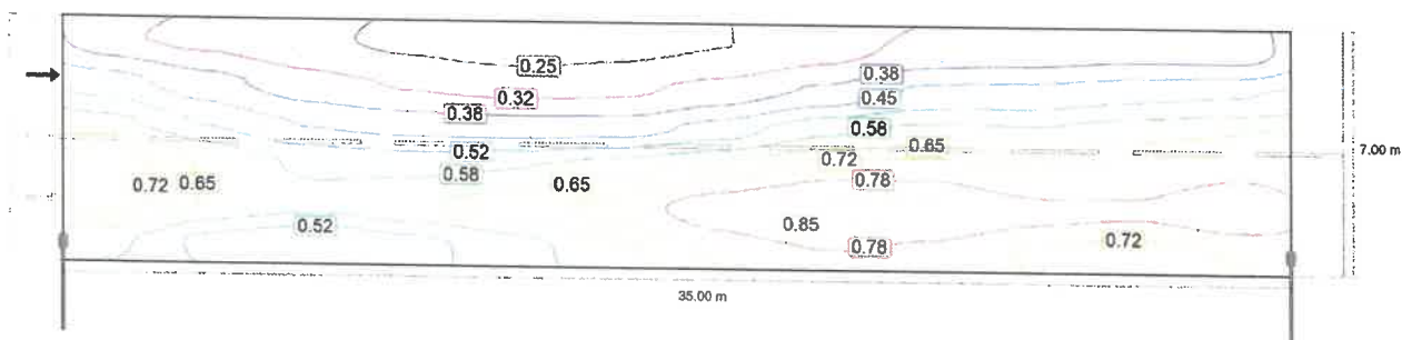
Observer 2: Maintenance value, luminance with dry roadway [ \text{cd/m}^2 ] (Iso-illuminance curves)
