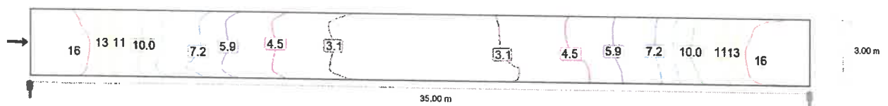
Maintenance value, horizontal illuminance [lx] (Iso-illuminance curves)
