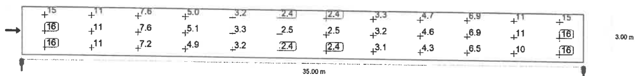
Maintenance value, horizontal illuminance [lx] (Value grid)
